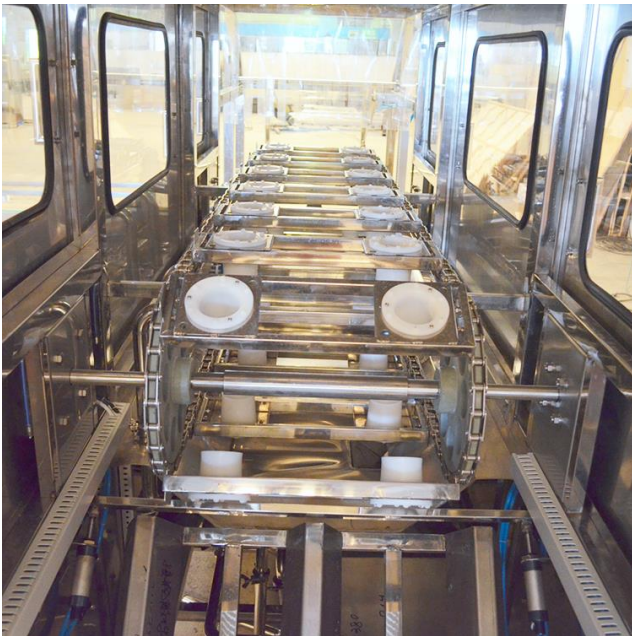
Washing Units
