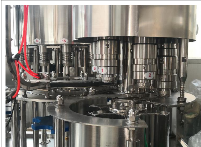
Capping Head
